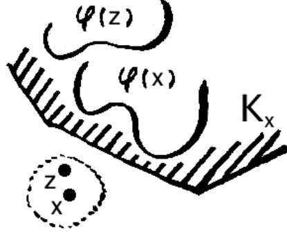
Figure 14: Mappings of Class \mathcal{H} and \mathcal{D}
